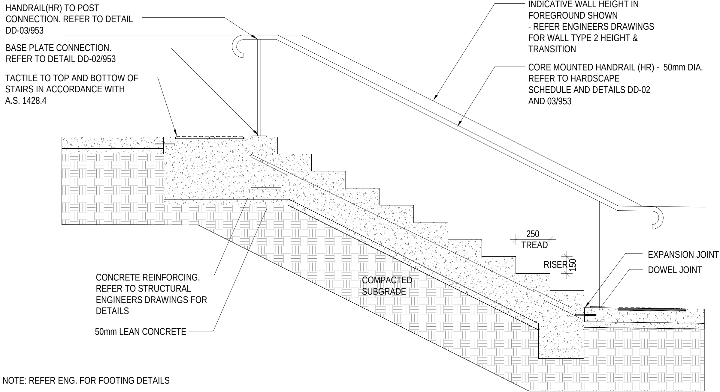
1 STR - INSITU CONCRETE STAIR - TYPICAL DETAIL SCALE - 1 : 20
